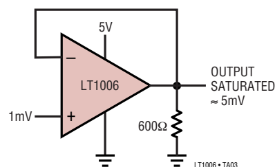
Voltage Follower
