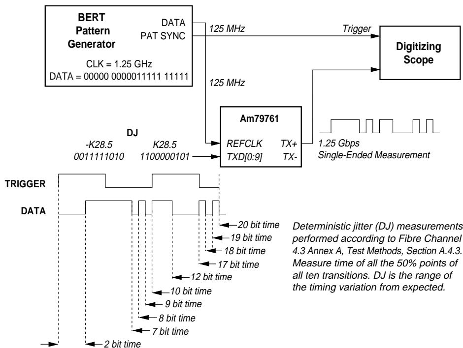
Figure 25. Transmitter Jitter Measurement Method
