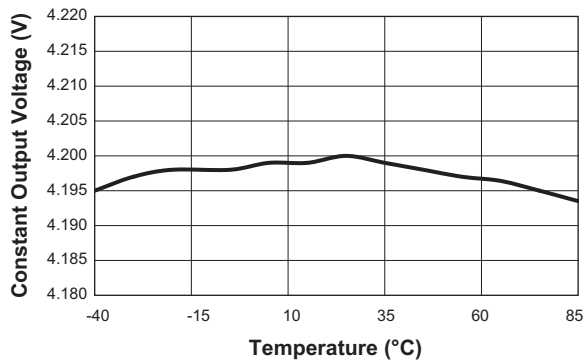
Constant Output Voltage vs. Temperature (R SET = 1.58KΩ)
