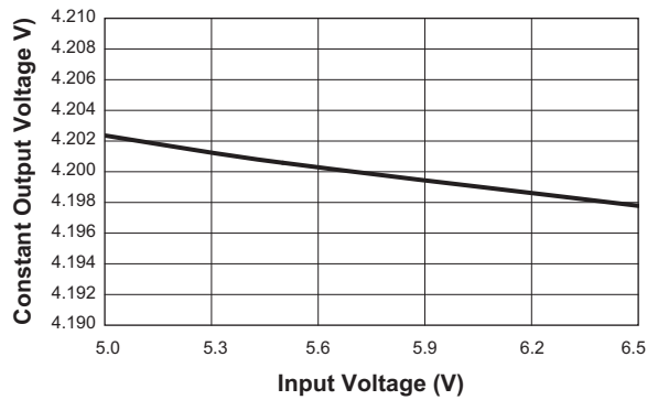
Constant Output Voltage vs. Input Voltage (R SET = 1.58KΩ)
