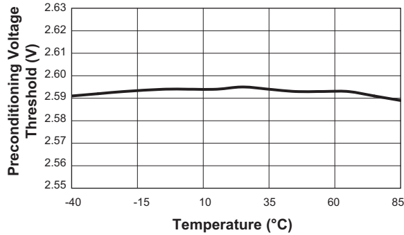
Preconditioning Voltage Threshold vs. Temperature (R SET = 1.58KΩ)
