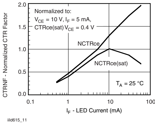
Fig. 11 - Normalization Factor for Non-Saturated and Saturated CTR vs. I F
