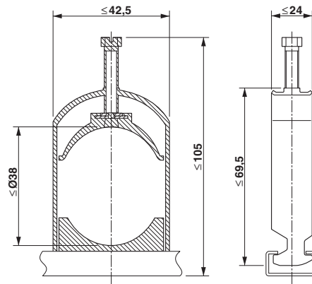
Dimensioned drawing
