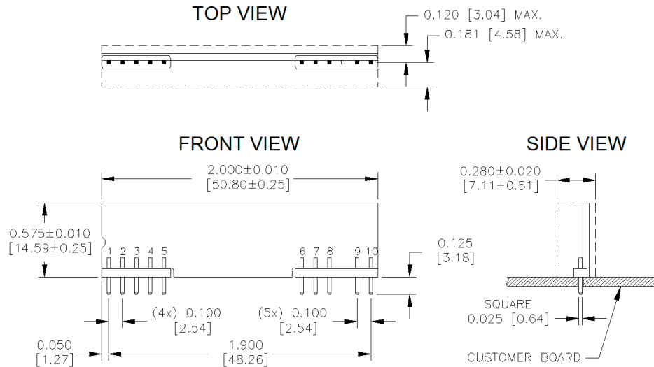
YNV05T10 Pinout (Through-Hole - SIP)
