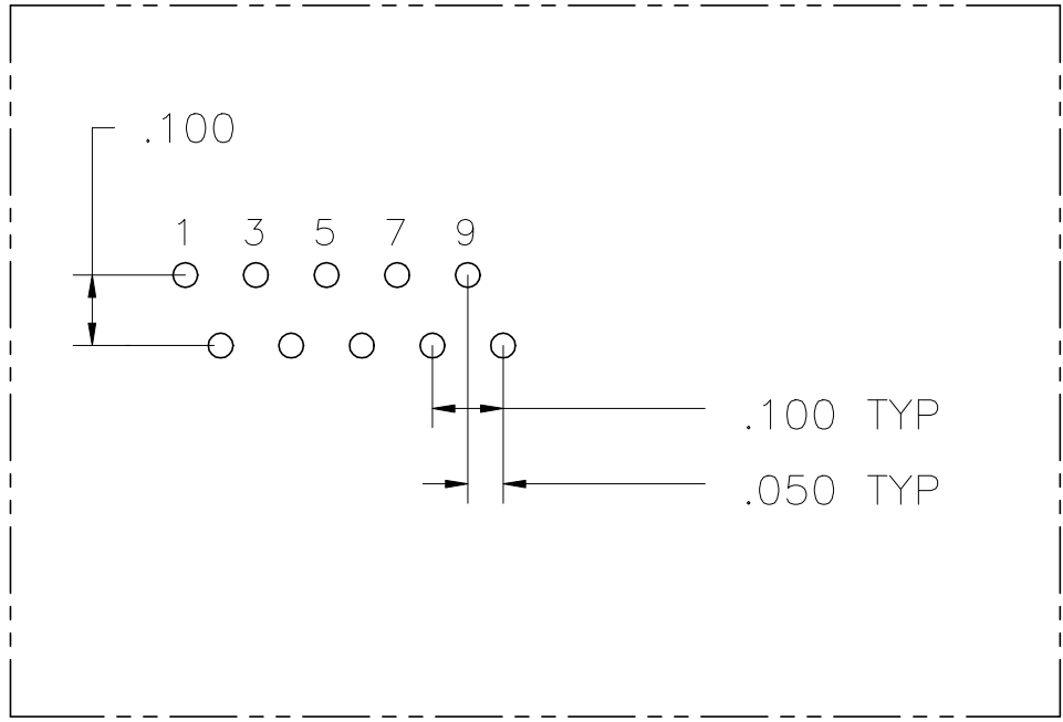
Pin Designations
