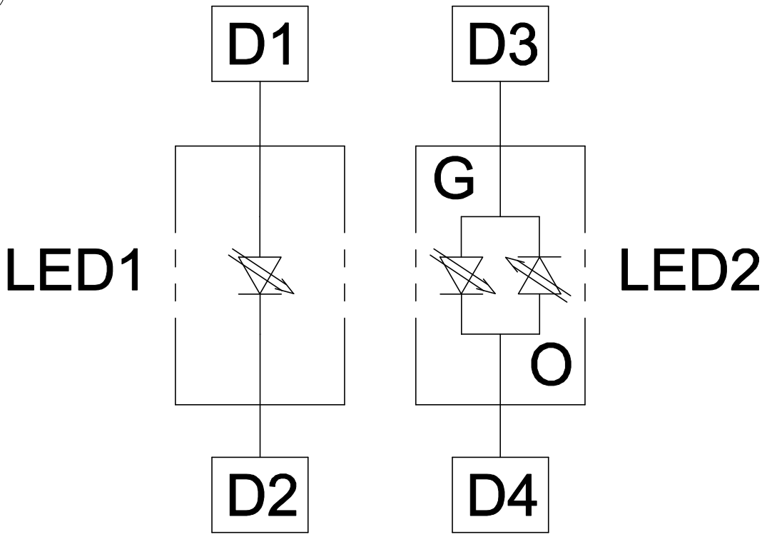
LED CONFIGURATION FOR 1-6605444-8 ONLY
