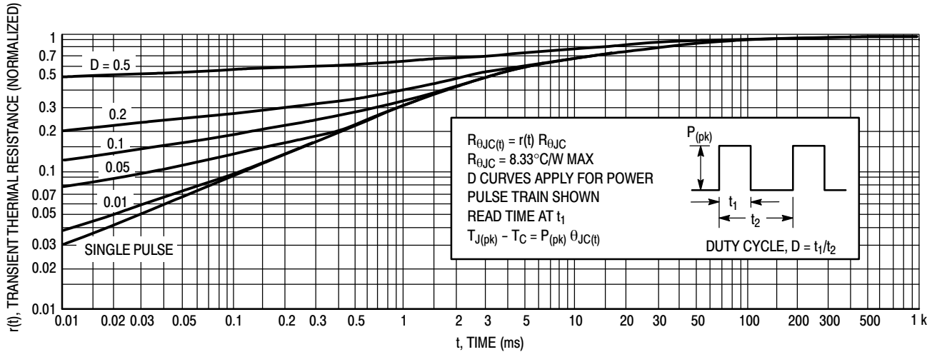
Figure 5. Thermal Response
