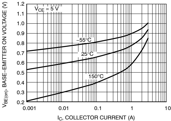
Figure 10. Base-Emitt "On" Voltage
