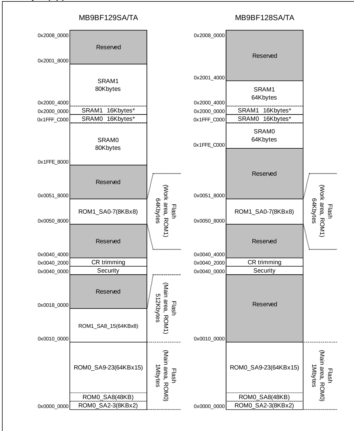
Memory Map (2)
