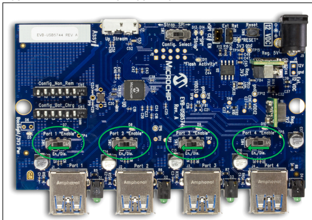
FIGURE 2-4: INITIAL CONFIGURATION
