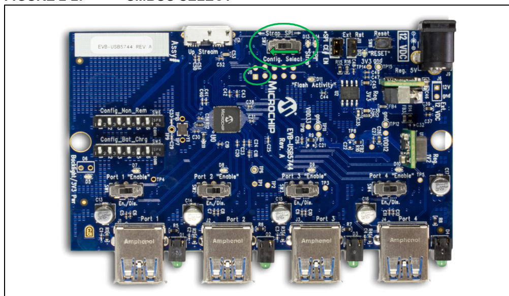
FIGURE 2-2: SMBUS SELECT
