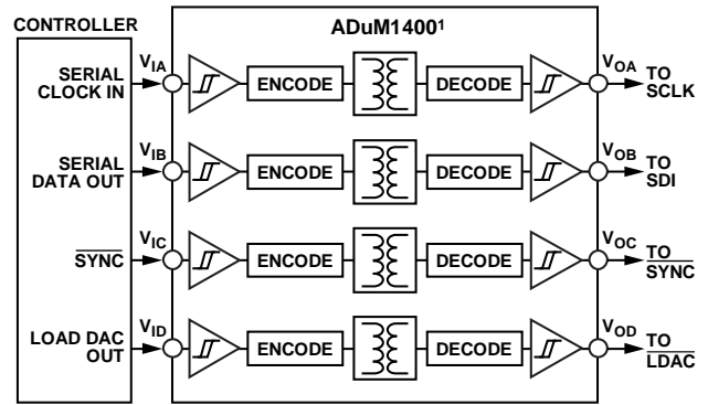
Figure 72. Isolated Interface
