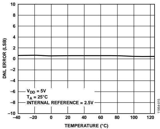
Figure 16. AD5676R DNL Error vs. Temperature
