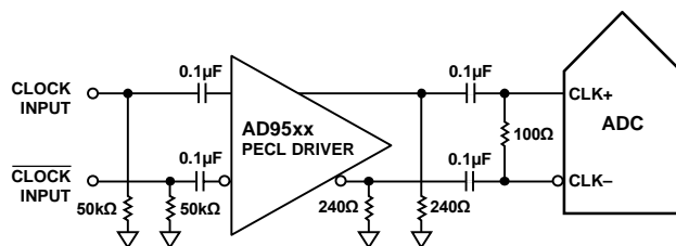
Figure 56. Differential PECL Sample Clock (Up to 640 MHz)
