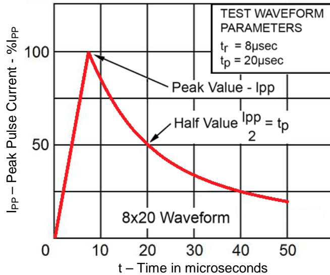
FIGURE 2 Pulse Waveform
