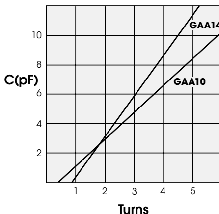
Capacitance vs. Rotation
