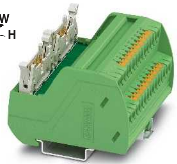
Passive interface modules for SIMATIC® S7-300 with push-in connection
