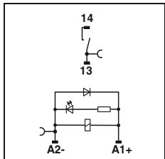
DC coils
