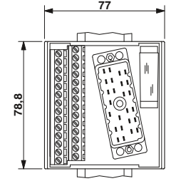
Dimensional drawing for UMK-EC56/25/EX-R
