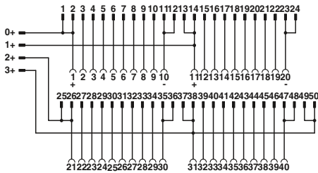
Connection scheme FLKM 50-PA-AB/OBN
