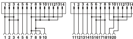
Connection scheme: FLKM 14-PA-AB/1756/IF6/EXTC
