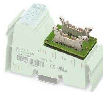
Front adapters for Inline
