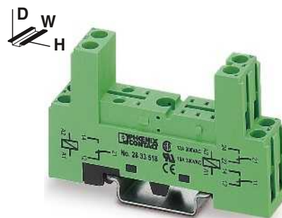
2/2-level design with screw connection
