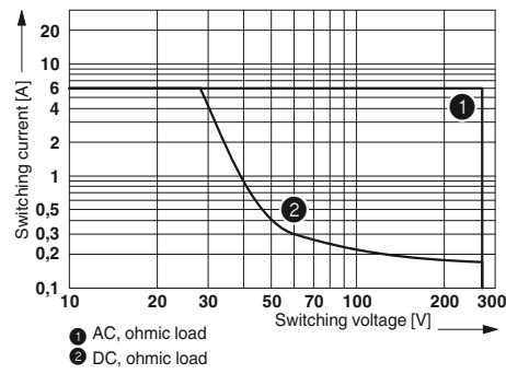
Interrupting rating
