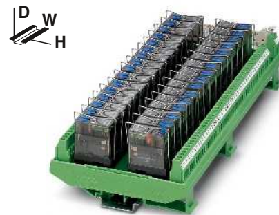
Output module with 32 miniature relays, 1 PDT with detectable manual operation
