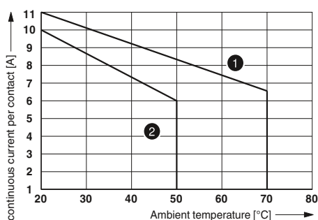
Contact derating
