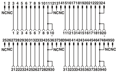
Connection scheme FLKM 50-PA-AB/IBN
