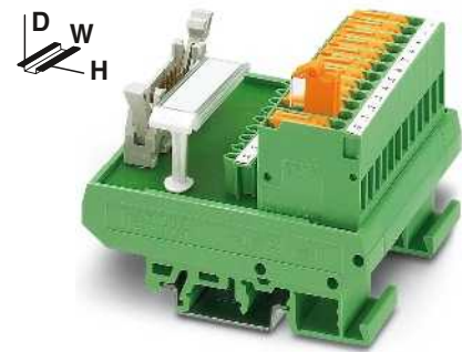
Passive interface modules for 8 or 32 channels with knife disconnect terminal blocks
