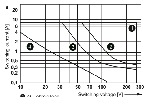
Interrupting rating
