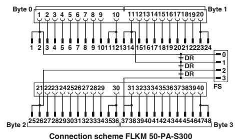
Connection scheme FLKM 50-PA-S300
