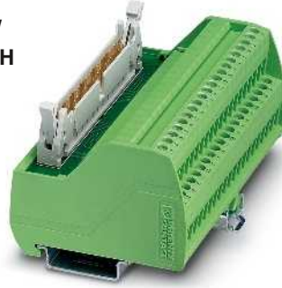
Passive interface modules for input/output, with SIMATIC®-specific marking and screw connection
