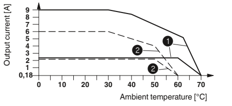
Derating curve ELR H3-IES-SC-230AC/500AC-2 and ELR H3-IES-SC-230AC/500AC-9 100% operating time
