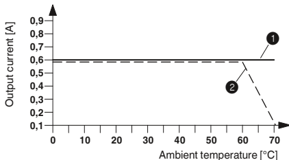
Derating curve ELR H3-IES-SC-24DC/500AC-0,6 100% operating time
