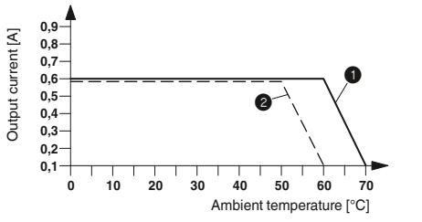
Derating curve ELR H5-IES-SC-230AC/500AC-0,6 100% operating time
