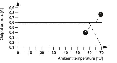
Derating curve ELR H5-IES-SC-24DC/500AC-0,6 100% operating time
