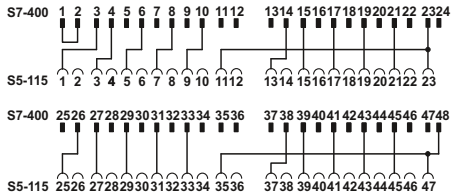
FLKM S115-454-7LA/S400 connection scheme
