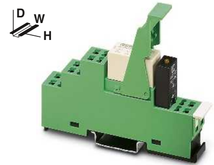
PR1 relay module with 1 PDT relay
