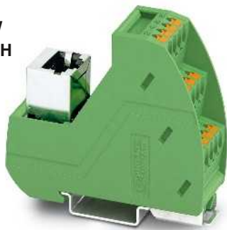
8-pos. with push-in connection
