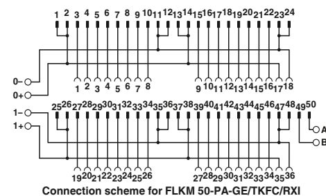
Connection scheme for FLKM 50-PA-GE/TKFC/RXI
