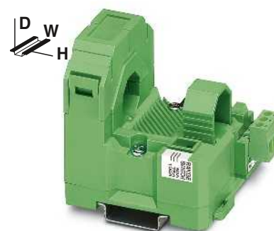
For sinusoidal and non-sinusoidal alternating currents, 0 ... 200 A, current output (loop-powered)
