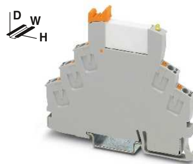
RIF-0 relay module with 1 PDT relay
