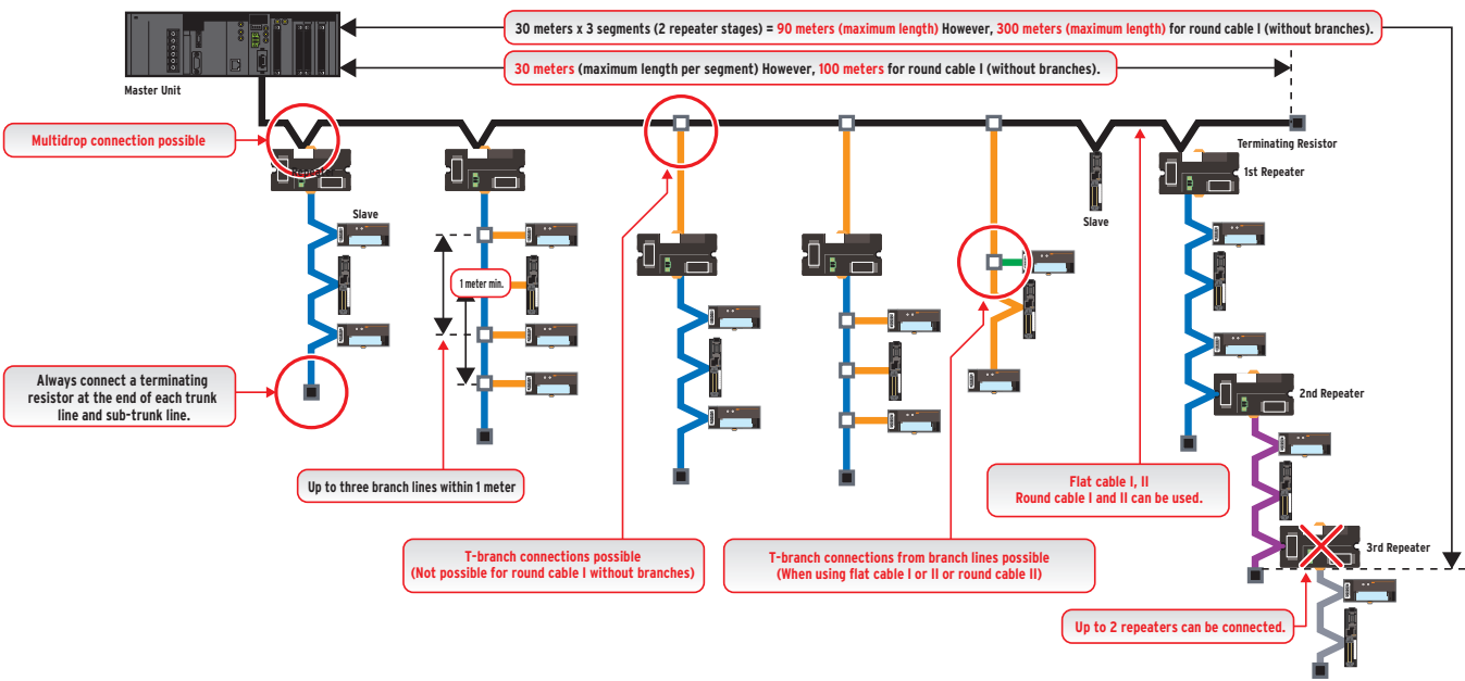
Example of wiring for 1.5 Mbps (Application: Balance of fast communications and branching)
