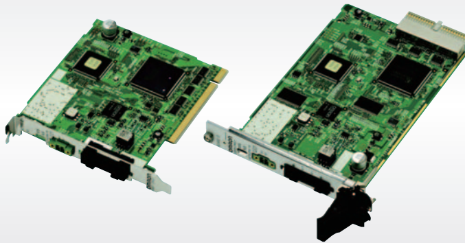
CompoNet Master Board for PCI Bus 3G8F7-CRM21
