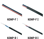
CompoNet Flat Cable I, II CompoNet Round Cable I, II ① CompoNet Flat Cable KOMP-F I 21AWG x 2, 19AWG x 2 ② CompoNet Flat Cable KOMP-F II 21AWG x 2, 19AWG x 2 ③ CompoNet Round Cable KOMP-R I 19AWG x 2 ④ CompoNet Round Cable KOMP-R II 19AWG x 4
