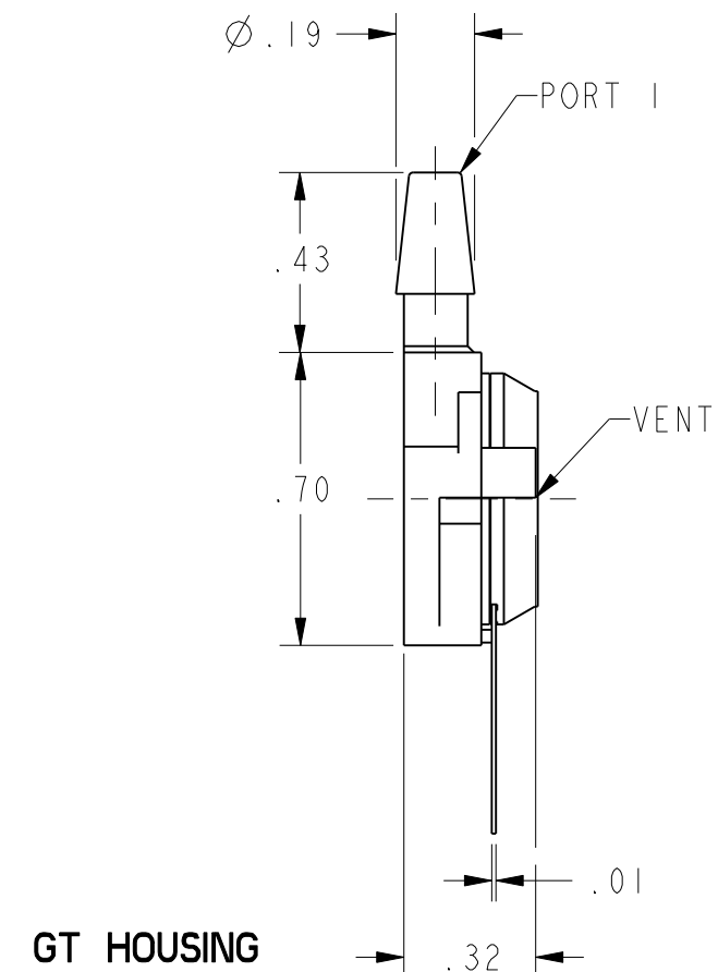
GT HOUSING
