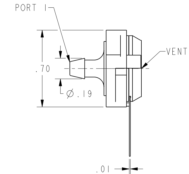
GF HOUSING
