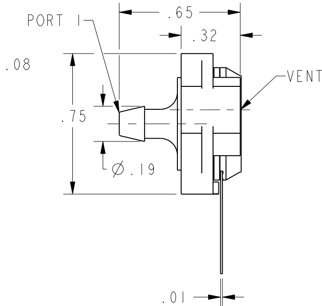
GFS HOUSING
