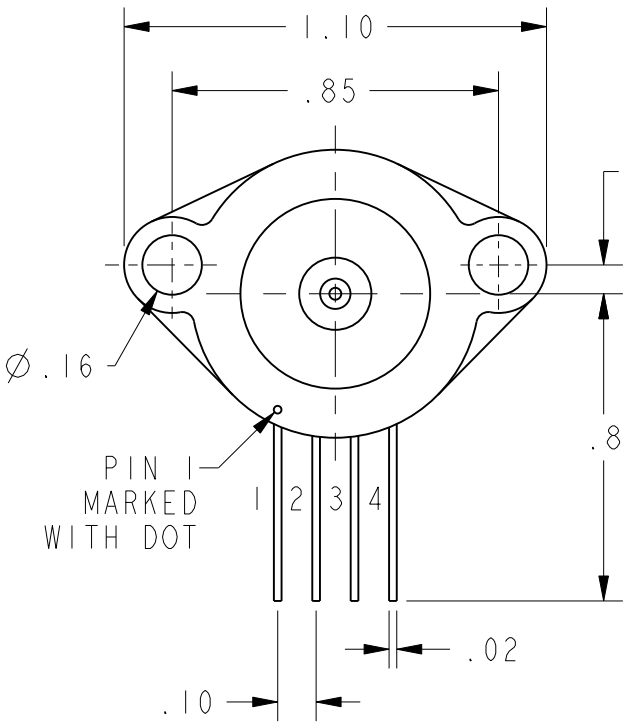
GFS HOUSING
