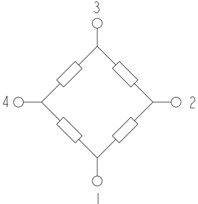
EQUIVALENT CIRCUIT
