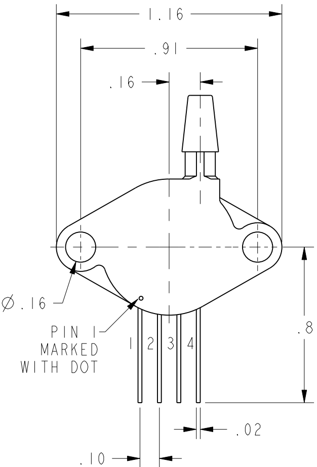
GT HOUSING
