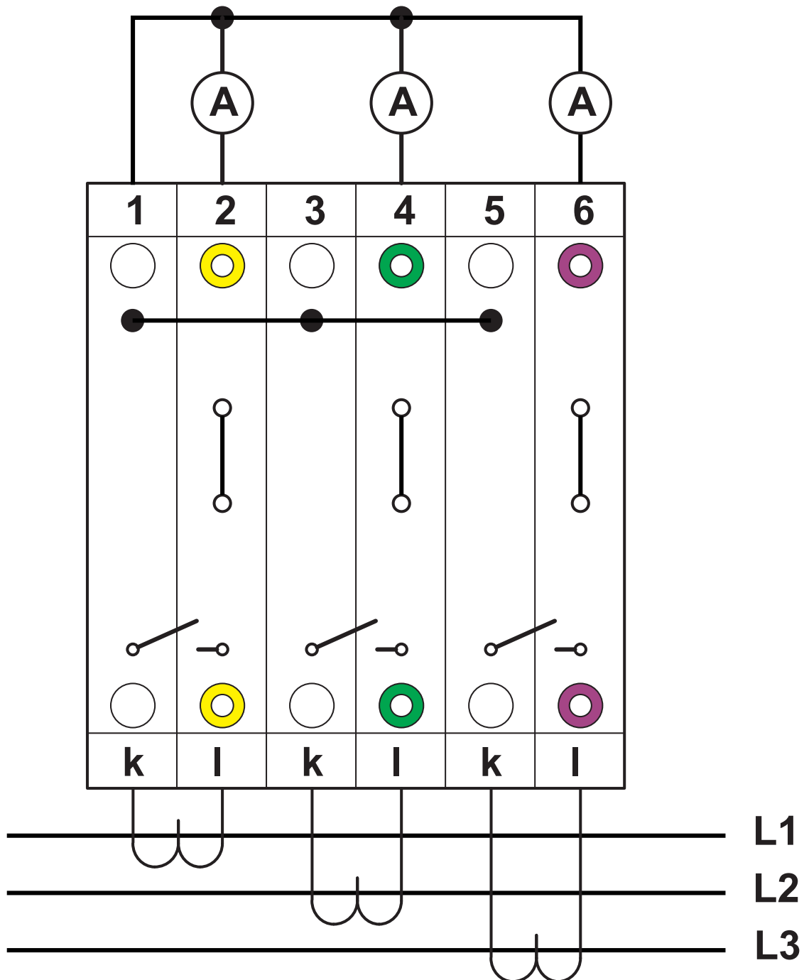
Connection diagram
