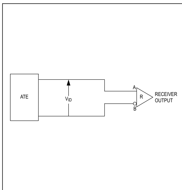
Figure 6. Receiver Propagation Delay Test Circuit
