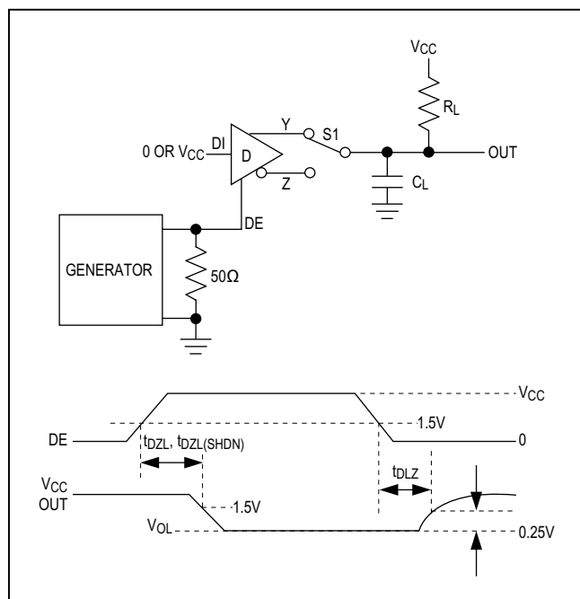
Figure 5. Driver Enable and Disable Times ( t_{DZL} , t_{DZ} , t_{DZL(SHDN)} , t_{DZ(SHDN)} )
