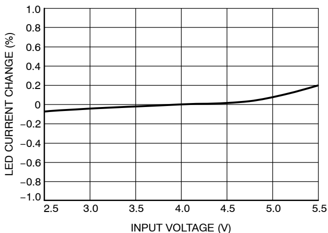
Figure 5. LED Current Change vs. Input Voltage
