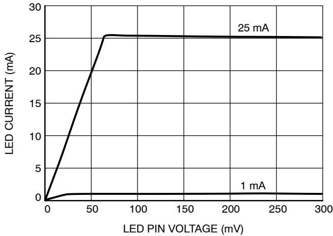
Figure 9. Dropout Characteristics
