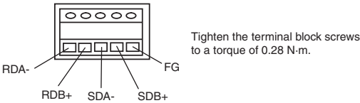
RS-422A/485 Connector
