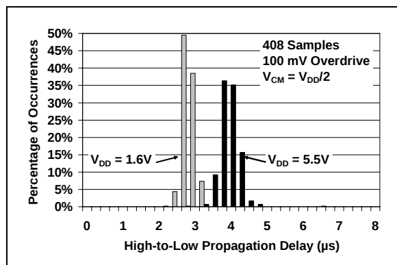
FIGURE 2-25: High-to-Low Propagation Delay.
