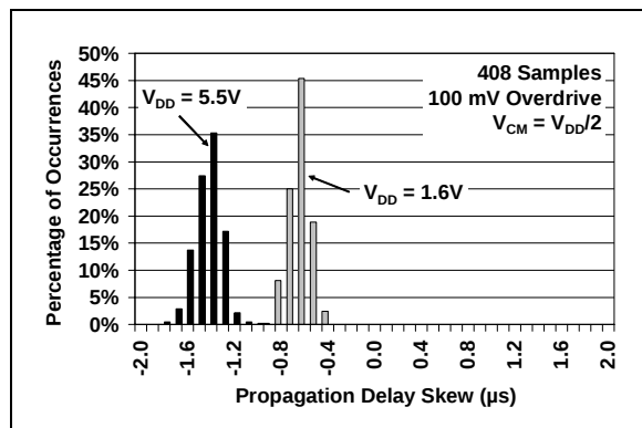
FIGURE 2-26: Propagation Delay Skew.
