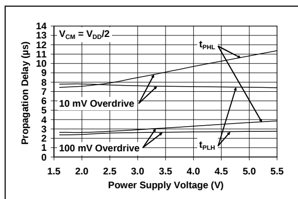
FIGURE 2-27: Propagation Delay vs. Power Supply Voltage.
