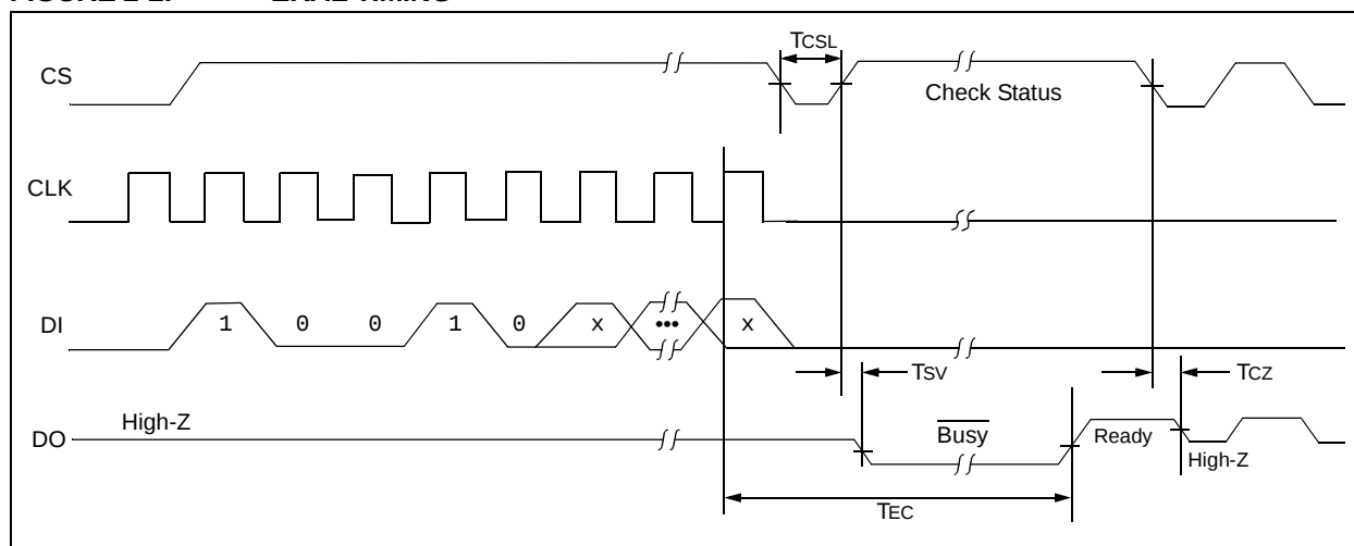
FIGURE 2-2: ERAL TIMING
