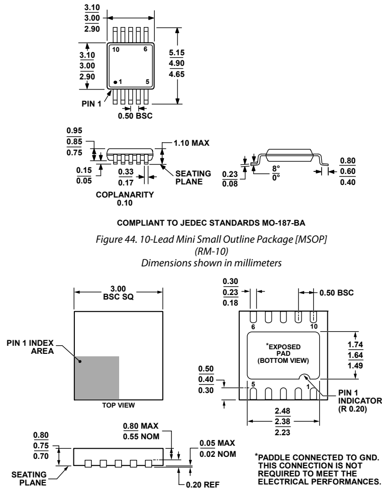
Figure 45. 10-Lead Lead Frame Chip Scale Package [LFCSP_WD] 3 mm x 3 mm Body, Very, Very Thin, Dual Lead (CP-10-9)
