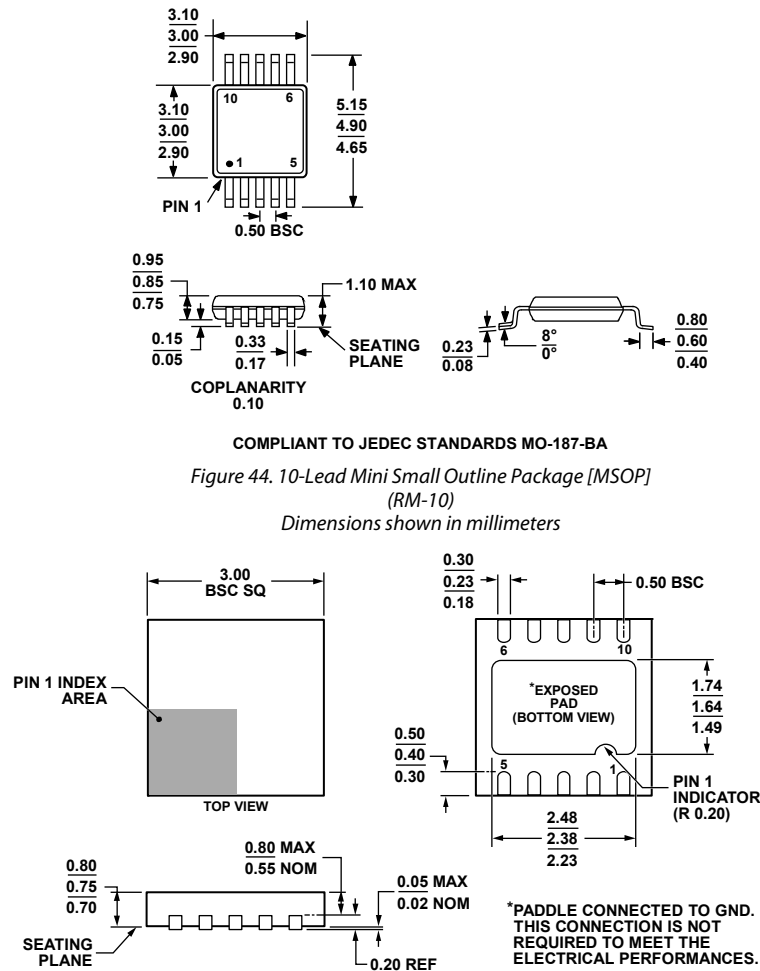
Figure 45. 10-Lead Lead Frame Chip Scale Package [LFCSP_WD] 3 mm × 3 mm Body, Very, Very Thin, Dual Lead (CP-10-9)
