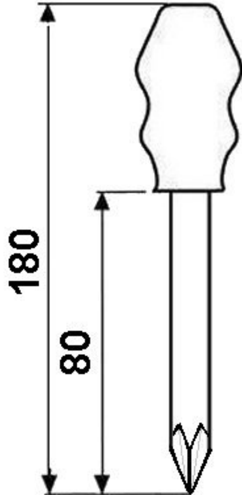
Dimensioned drawing
