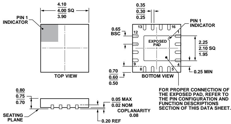
COMPLIANT TO JEDEC STANDARDS MO-220-WGGC. Figure 66. 16-Lead Lead Frame Chip Scale Package [LFCSP_WQ] 4 mm × 4 mm Body, Very Very Thin Quad (CP-16-23) Dimensions shown in millimeters
