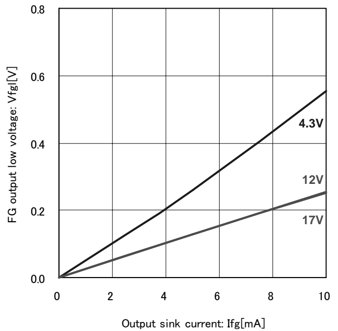
Fig.14 FG output low voltage (Ta=25°C)
