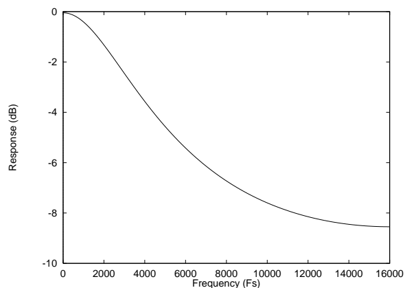
Figure 43 De-emphasis Frequency Response (32kHz)
