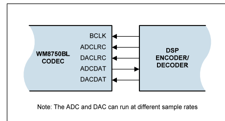
Figure 17 Slave Mode
