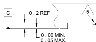
DETAIL "X"
