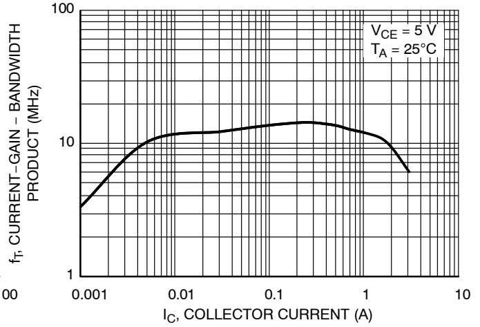
Figure 13. Current-Gain-Bandwidth Product
