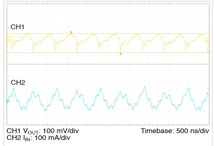
Figure 11 — Full load ripple, 2700 \mu F C_{PRI\_IN\_EXT} ; No external C_{SEC\_OUT\_EXT} . Board mounted module, scope setting : 20 MHz analog BW
