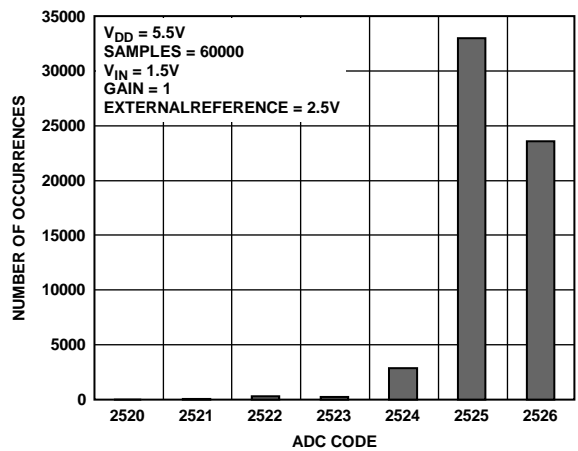
Figure 15. Histogram of ADC Codes, V_{DD} = 5.5\text{ V}
