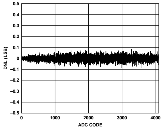
Figure 13. ADC DNL, V_{DD} = 2.7\text{ V}
