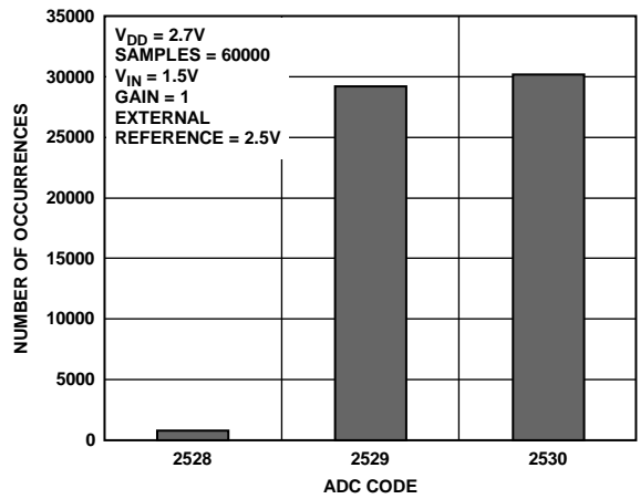
Figure 14. Histogram of ADC Codes, V_{DD} = 2.7\text{ V}
