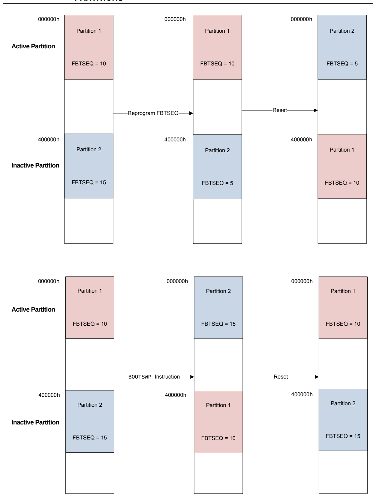
FIGURE 4-4: RELATIONSHIP BETWEEN PARTITIONS 1 AND 2 AND ACTIVE/INACTIVE PARTITIONS
