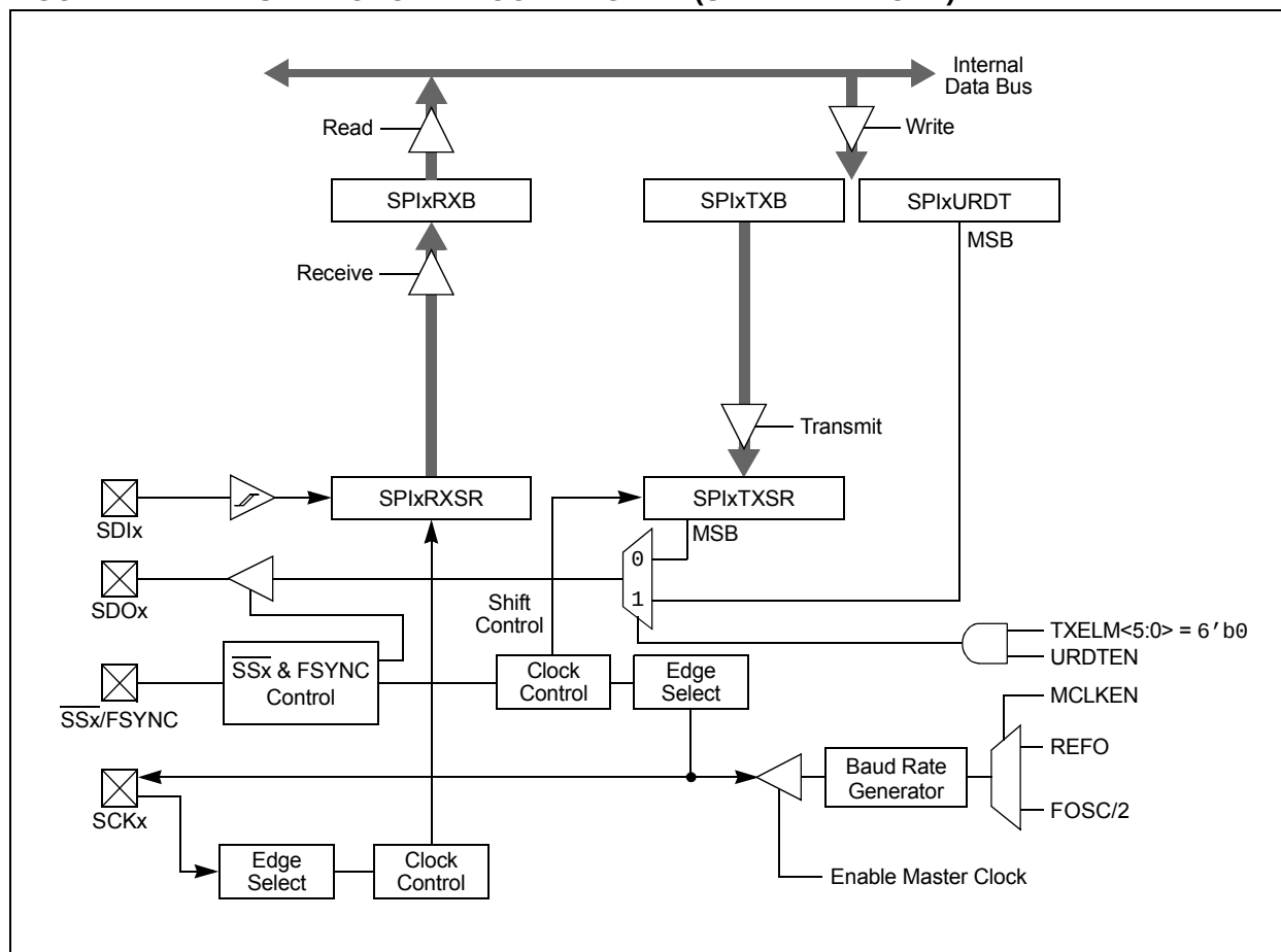
FIGURE 17-1: SPIx MODULE BLOCK DIAGRAM (STANDARD MODE)
