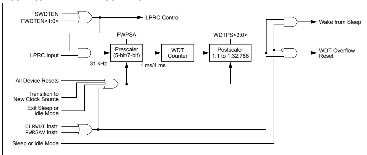
FIGURE 33-2: WDT BLOCK DIAGRAM
