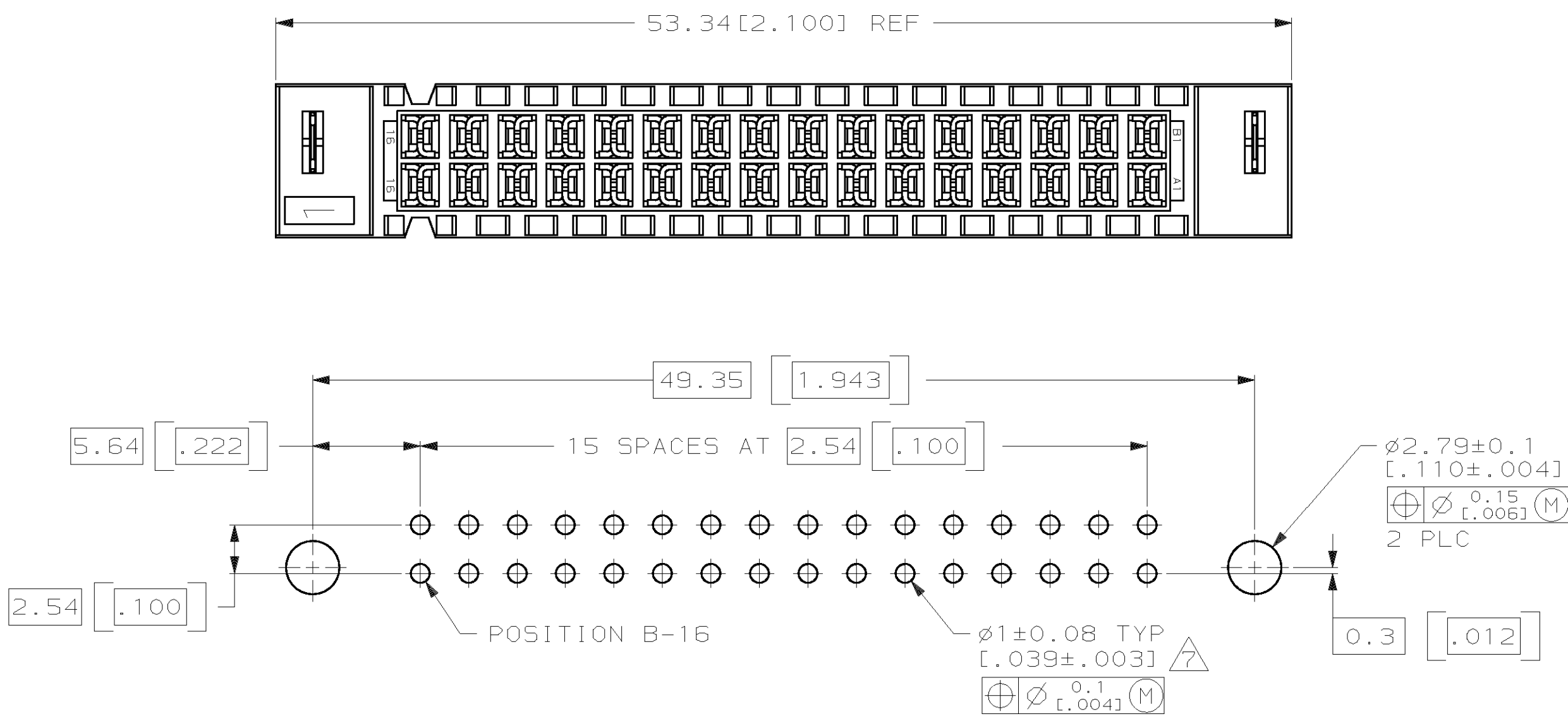
PC BOARD LAYOUT
