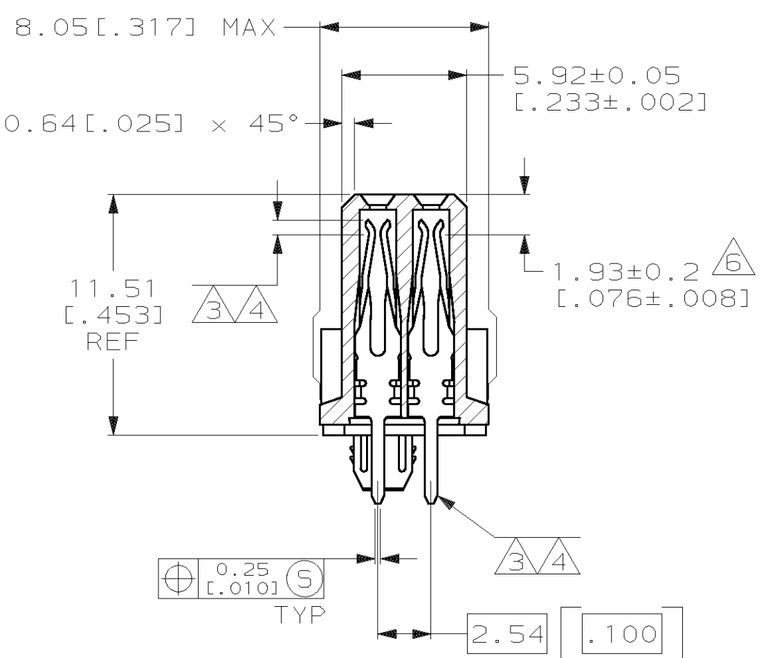
SECTION X-X
