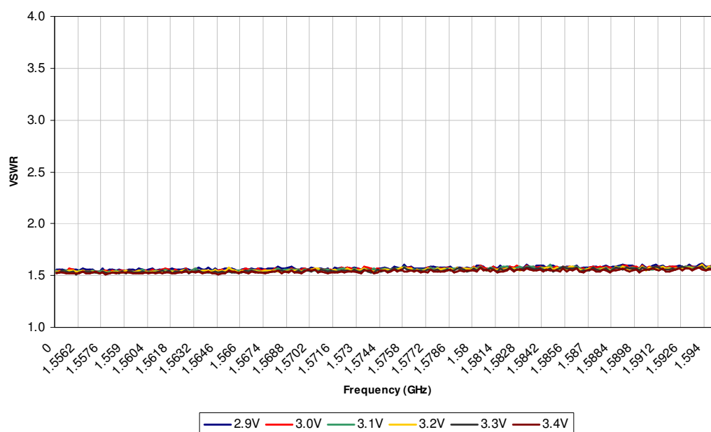
Fig 2: Output VSWR vs DC input voltage
