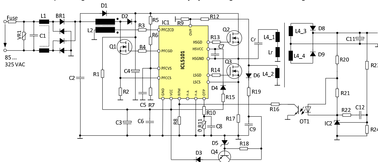
Figure 18 Principle Schematic ICL5101
