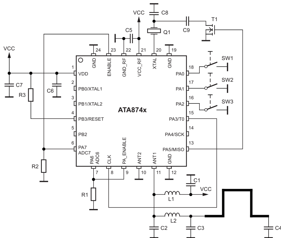
Figure 8-3. Typical FSK Application ATA8742
