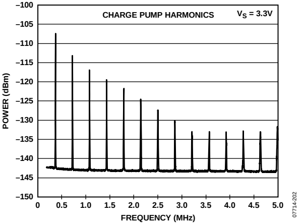
Figure 35. Output Spectrum vs. Frequency, V_S = 3.3\text{ V}
