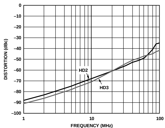
Figure 14. Harmonic Distortion vs. Frequency, V_S = 3.3V
